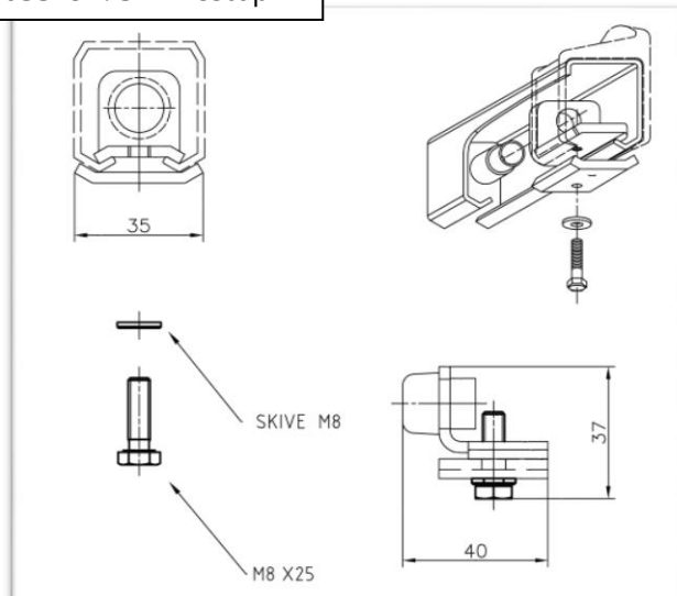
9033792: Skinnestop
