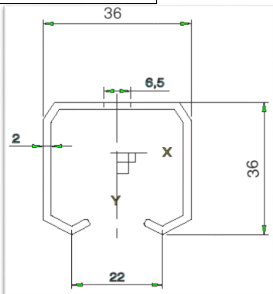
9014214: Port skinne
