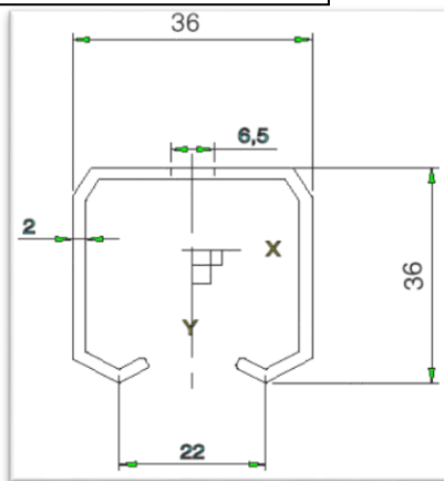
9056688: Port skinne
