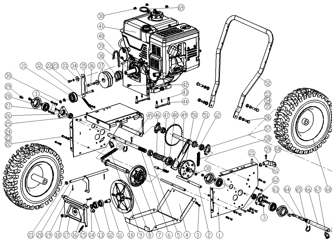
Fig. 3 Transmission
