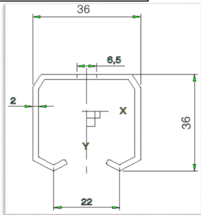
9054185: Port skinne
