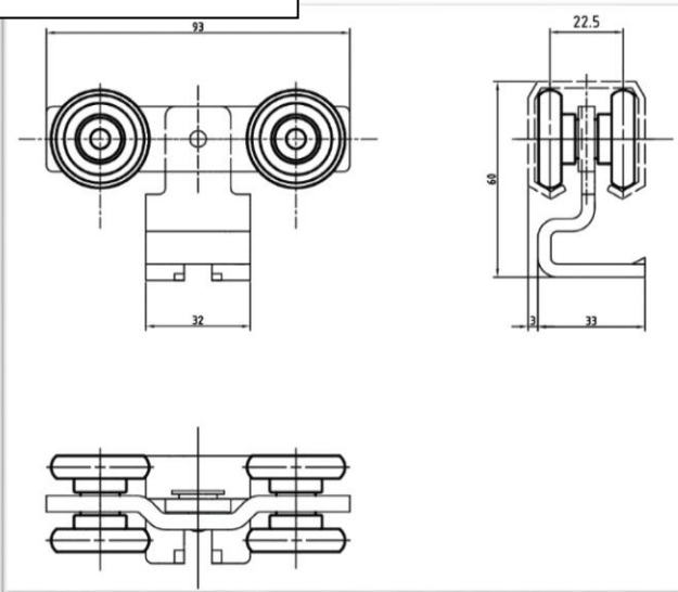
9056690: Port rulle
